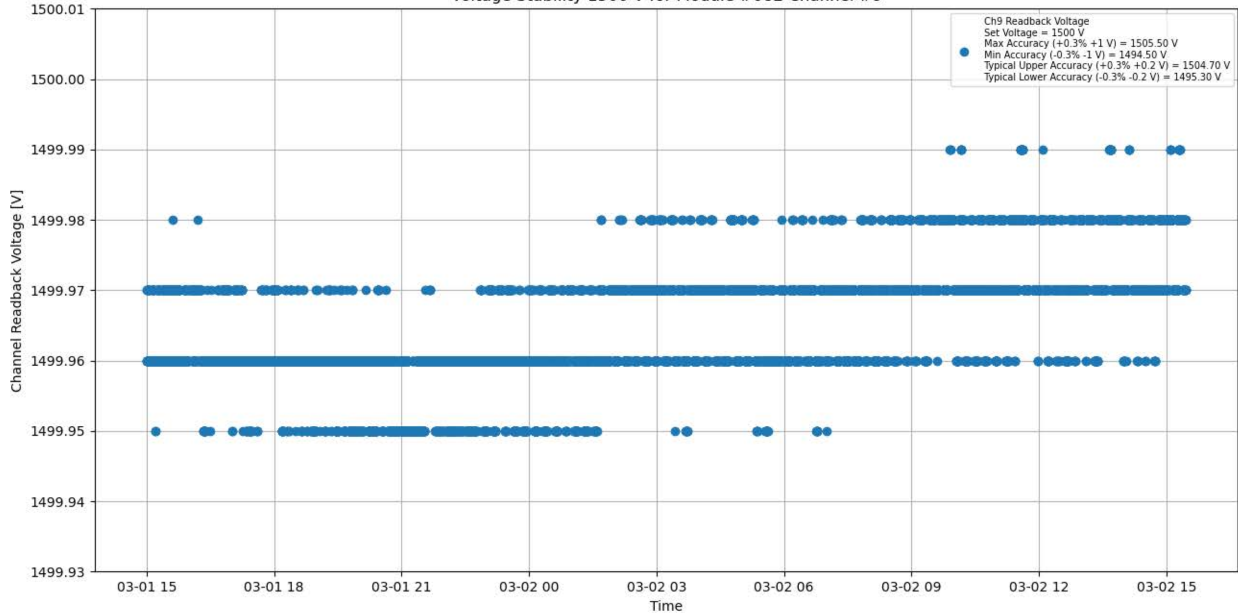
Voltage Stability 1500 V for Module #082 Channel #9
