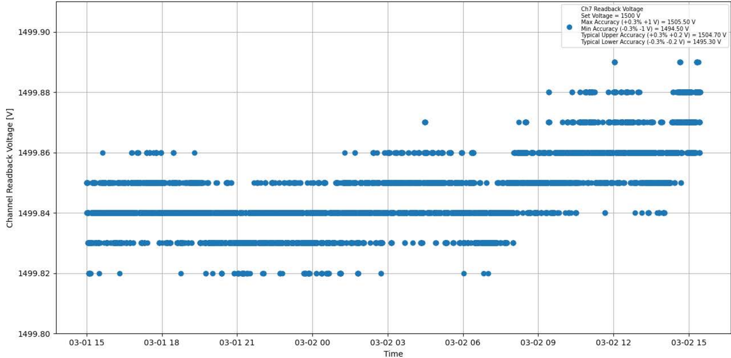
Voltage Stability 1500 V for Module #082 Channel #7
