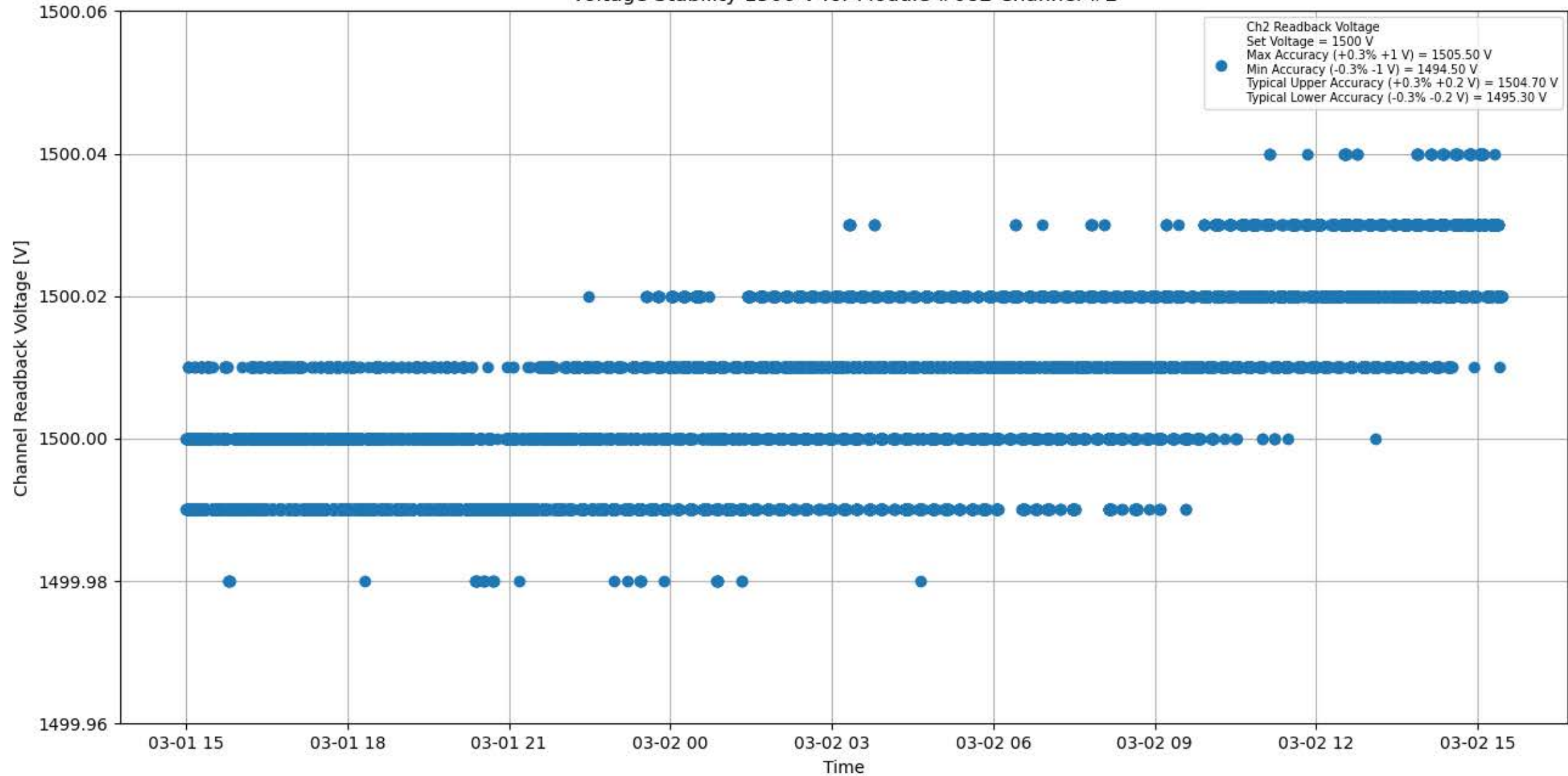
Voltage Stability 1500 V for Module #082 Channel #2
