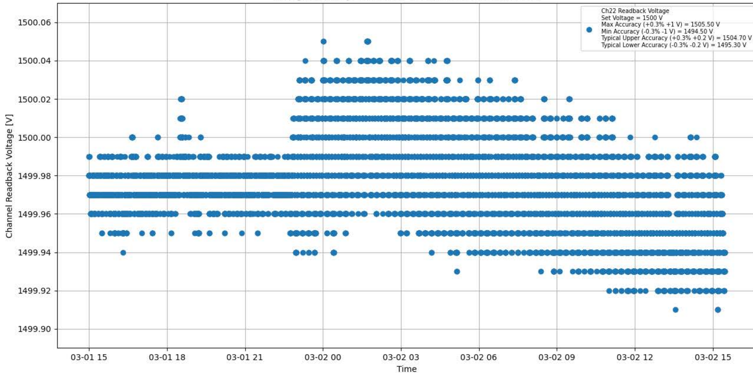
Voltage Stability 1500 V for Module #082 Channel #22
