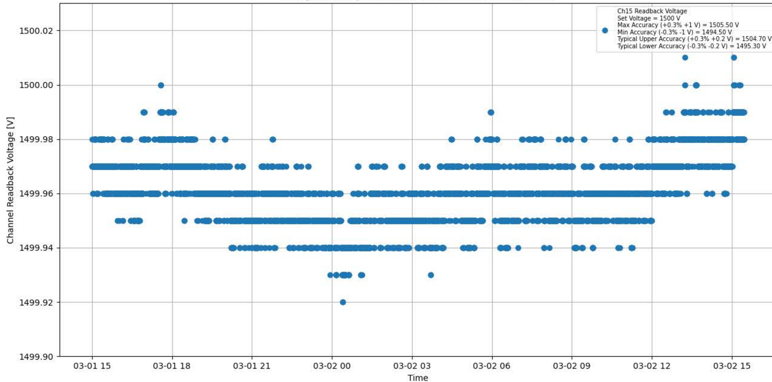
Voltage Stability 1500 V for Module #082 Channel #15
