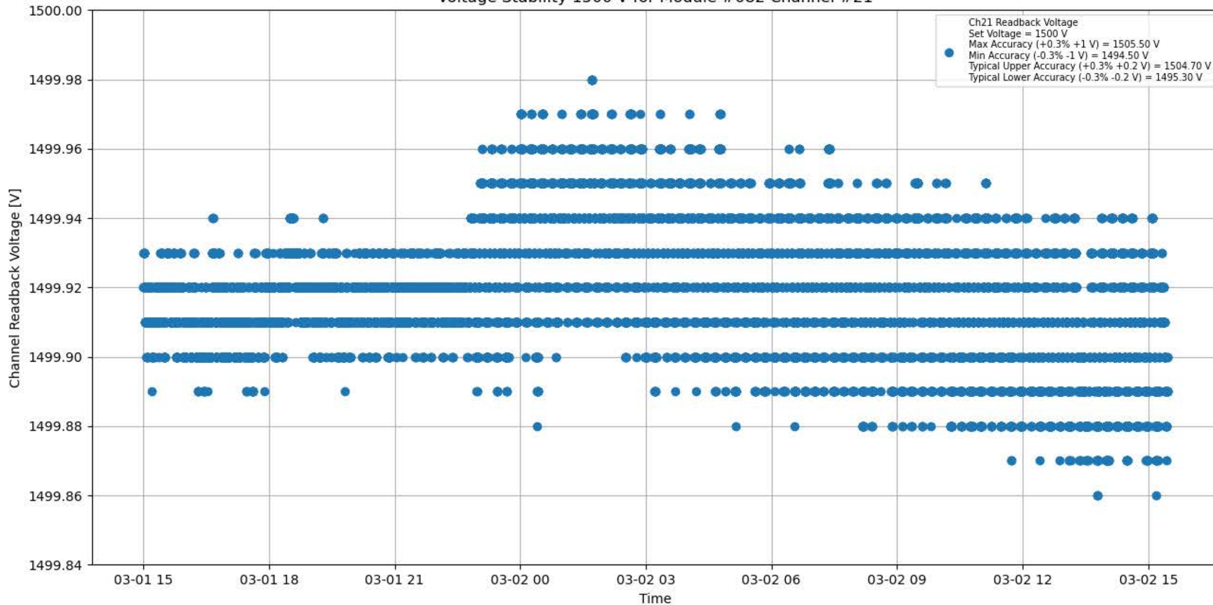
Voltage Stability 1500 V for Module #082 Channel #21
