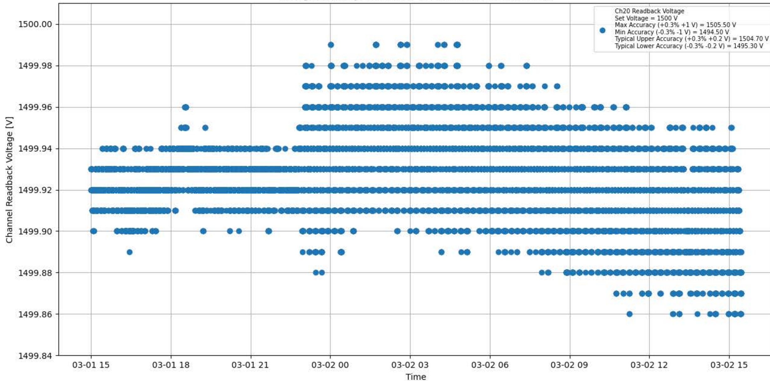
Voltage Stability 1500 V for Module #082 Channel #20
