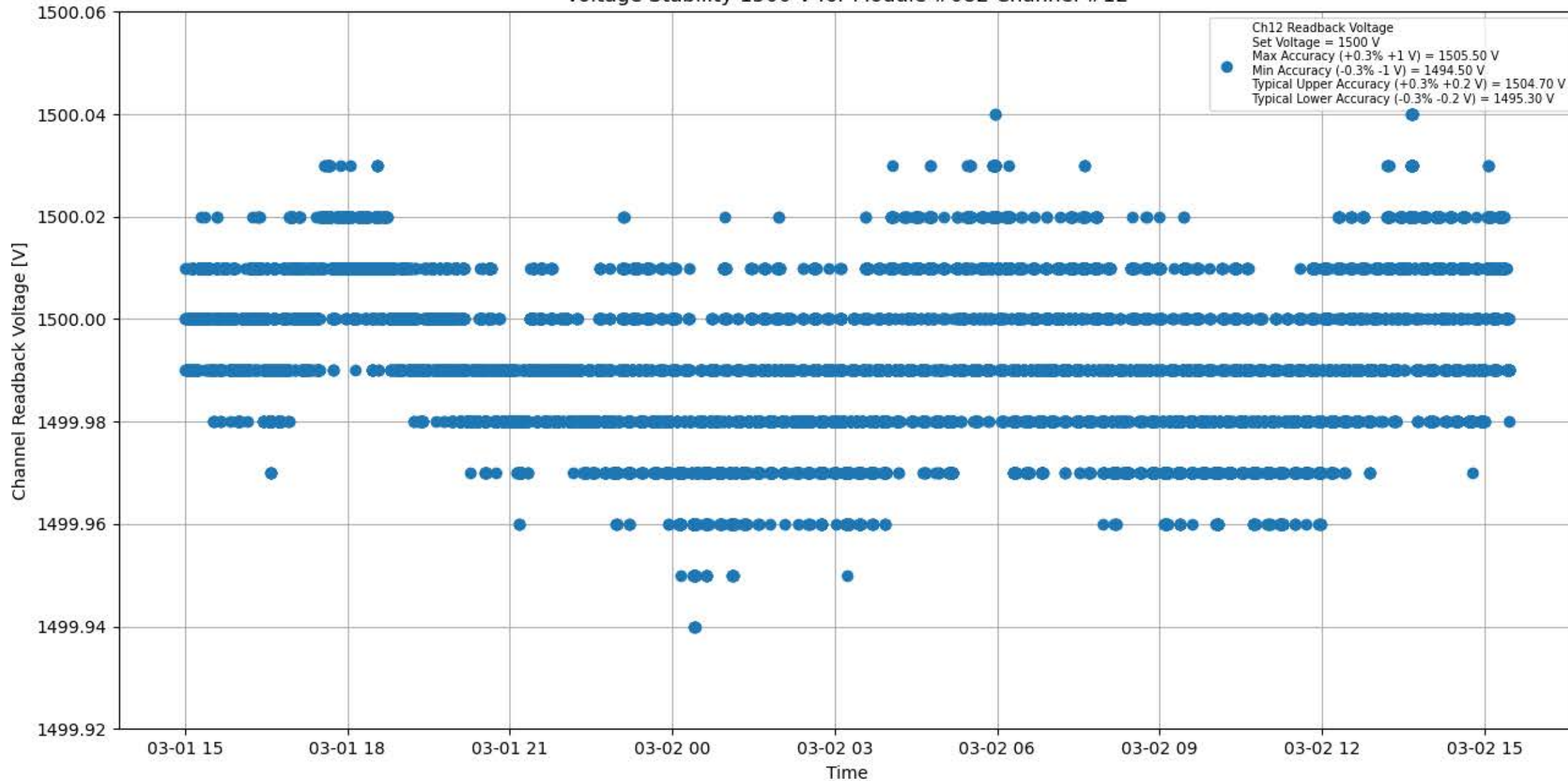
Voltage Stability 1500 V for Module #082 Channel #12
