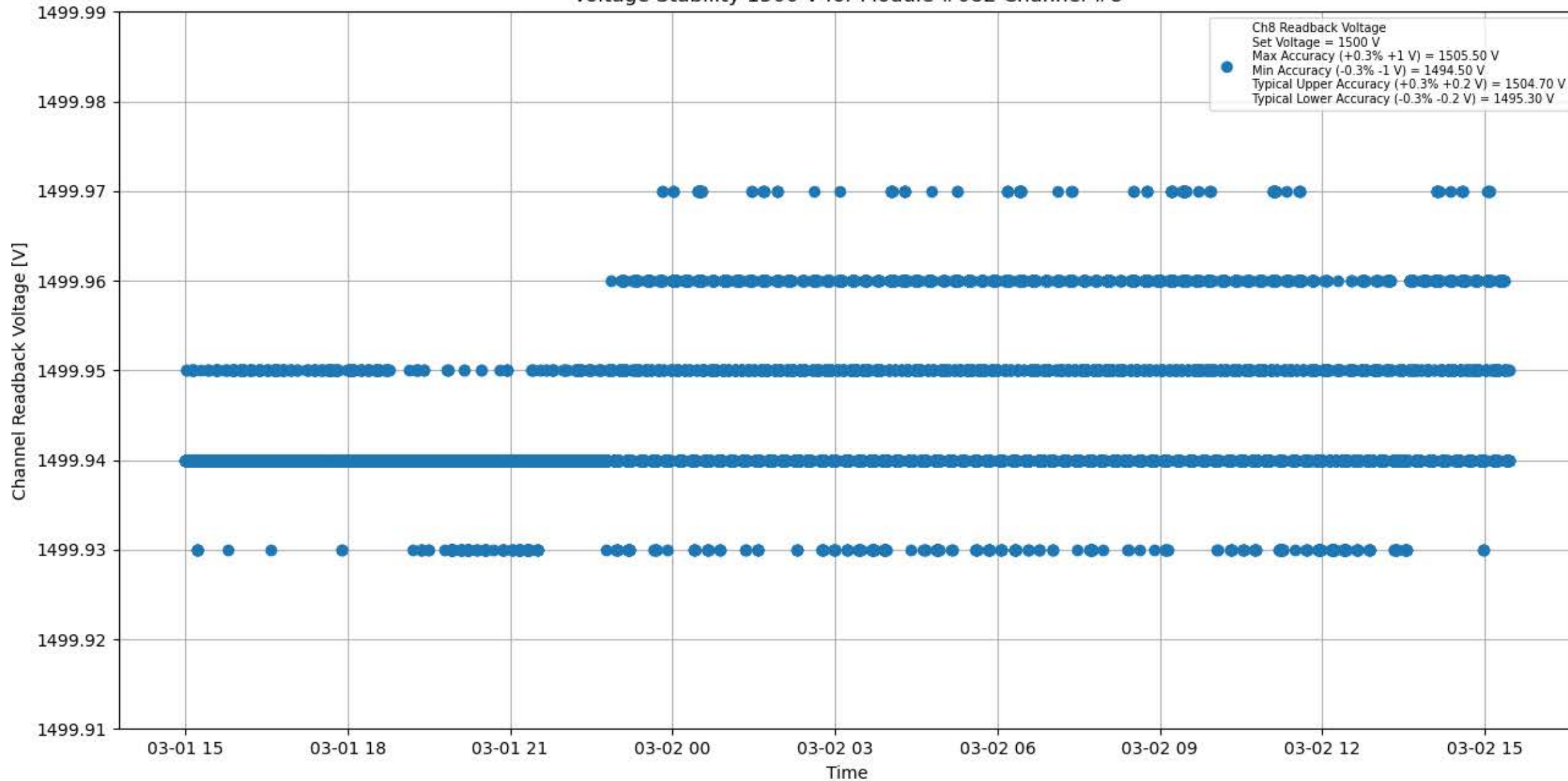
Voltage Stability 1500 V for Module #082 Channel #8
