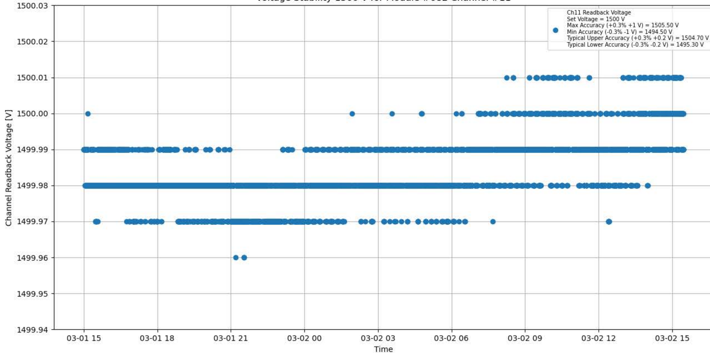
Voltage Stability 1500 V for Module #082 Channel #11
