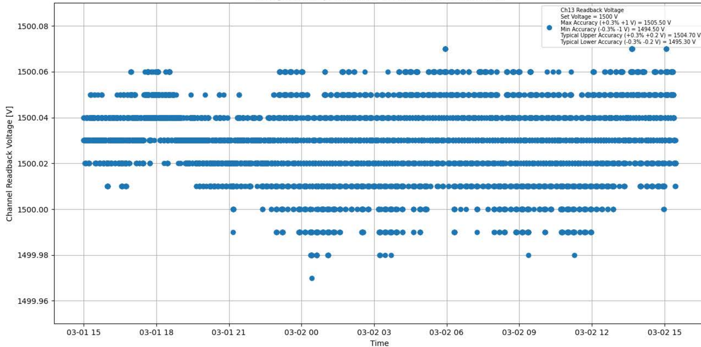
Voltage Stability 1500 V for Module #082 Channel #13
