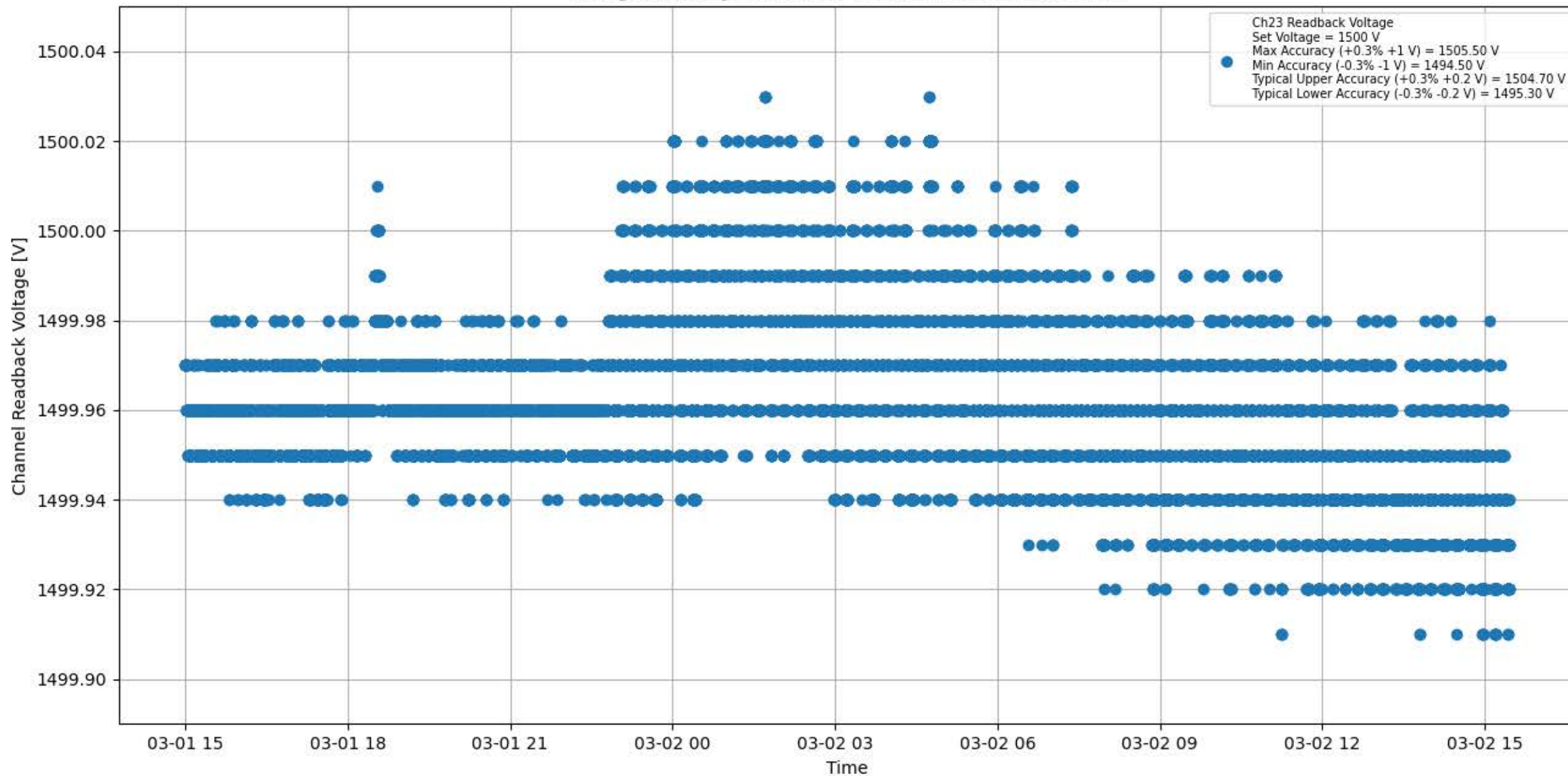
Voltage Stability 1500 V for Module #082 Channel #23
