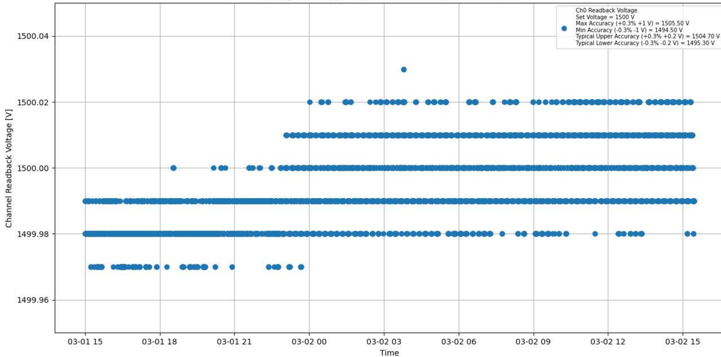
Voltage Stability 1500 V for Module #082 Channel #0
