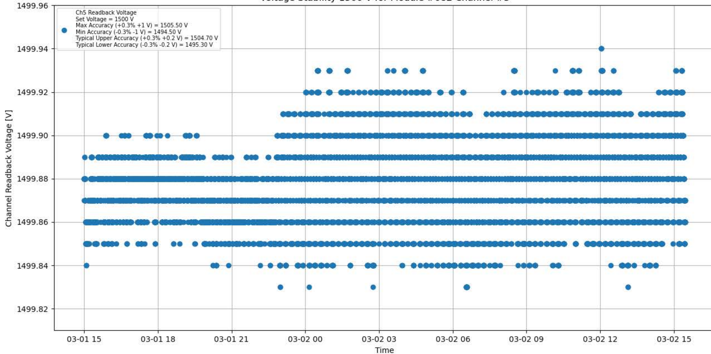
Voltage Stability 1500 V for Module #082 Channel #5
